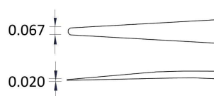
Dimensions inch
